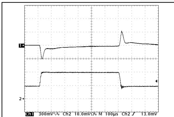
Figure 11: Output voltage response to step-change in load current (50%-100%-50% of Iout (max)). Load cap: 1µF ceramic cap and 10µF, 100 mΩ ESR tantalum cap. Ch 1: Vout (300mV/div). Ch 2: Iout (10A/div).
