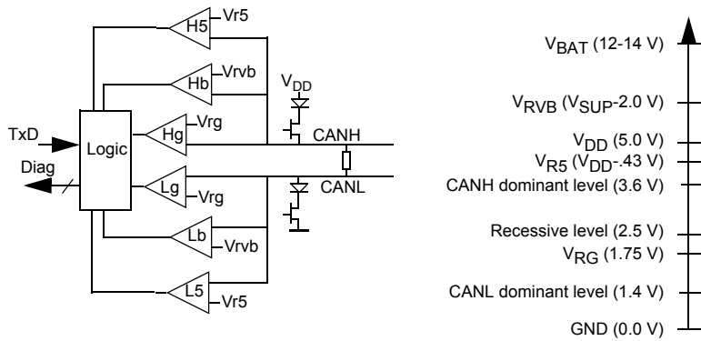
Figure 35. CAN Bus Simplified Structure Truth Table for Failure Detection
