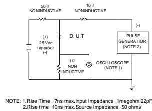
FIG.6-TEST CIRCUIT DIAGRAM AND REVERSE RECOVERY TIME CHARACTERISTIC
