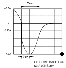
FIG.6-TEST CIRCUIT DIAGRAM AND REVERSE RECOVERY TIME CHARACTERISTIC
