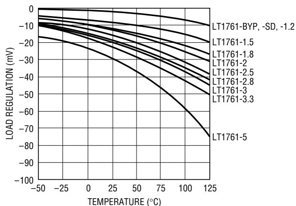
Load Regulation \Delta I_L = 1mA to 100mA
