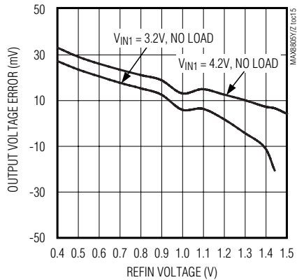
REFIN vs. REFIN TO OUT GAIN (MAX8805Y)
