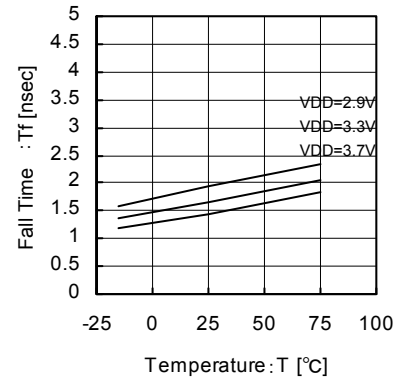
Fig.29 33.8688MHz Temperature - fall-time
