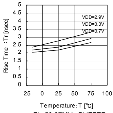
Fig.53 27MHz BUFFER Temperature - rise-time
