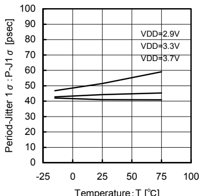
Fig.45 24.576MHz Temperature - Period-Jitter 1 sigma
