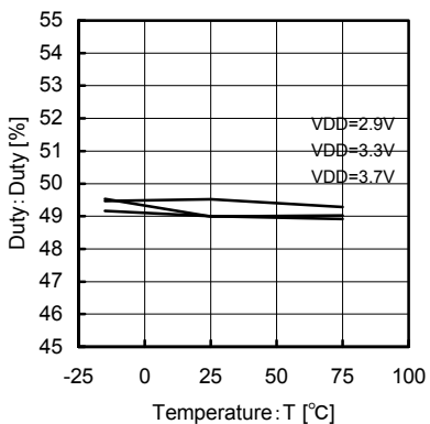
Fig.42 24.576MHz Temperature - Duty
