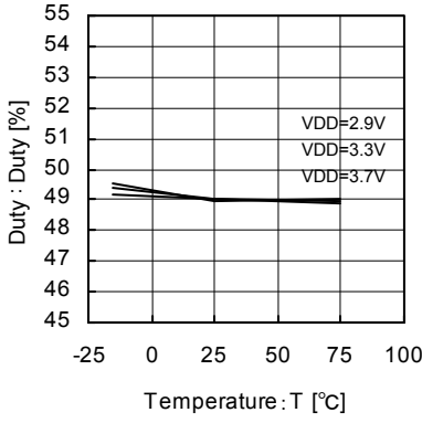
Fig.47 54MHz Temperature - Duty
