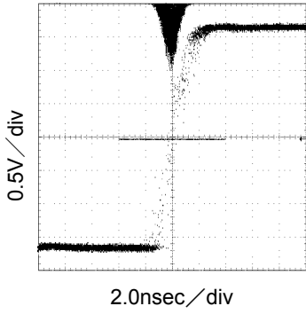
Fig.67 33.8688MHz Long Term Jitter
