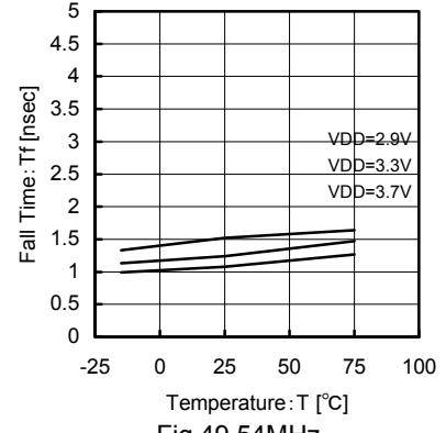
Fig.49 54MHz Temperature - fall-time
