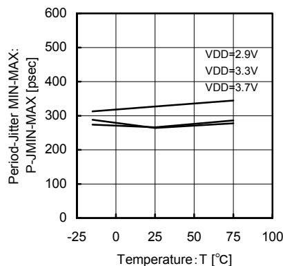
Fig.46 24.576MHz Temperature - Period-Jitter MIN-MAX
