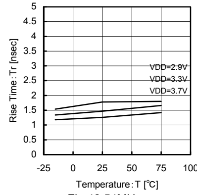
Fig.48 54MHz Temperature - rise-time
