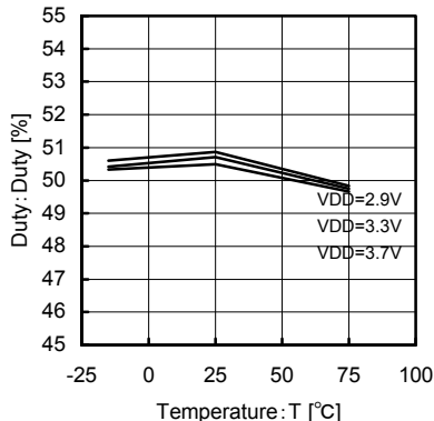
Fig.27 33.8688MHz Temperature - Duty
