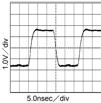
Fig.6 36.864MHz output waveform VDD=3.3V,CL=32pF
