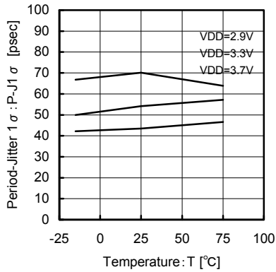
Fig.40 18.432MHz Temperature - Period-Jitter 1 sigma
