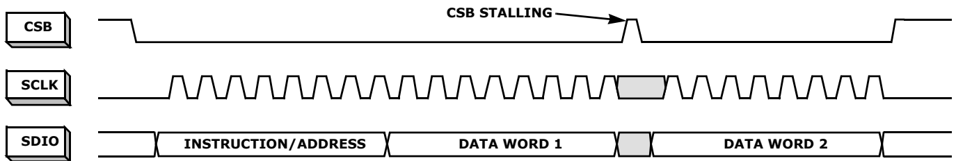
FIGURE 37. 2-BYTE TRANSFER
