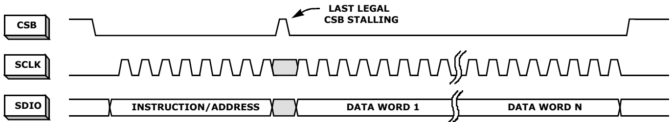
FIGURE 38. N-BYTE TRANSFER
