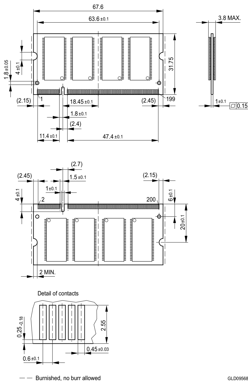
Package Outline SO-DIMM Raw Card A (L-DIM-200-6)
