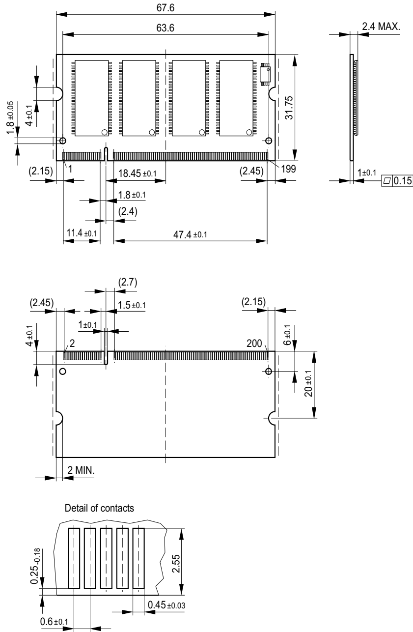
FIGURE 3 Package Outline SO-DIMM Raw Card C (L-DIM-200-11)
