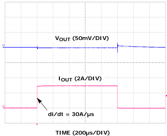
FIGURE 29. LOAD TRANSIENT 0A TO 3A, C_{OUT} = 10\mu F CERAMIC + 100µF OSCON
