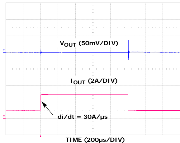
FIGURE 30. LOAD TRANSIENT 1A TO 3A, C_{OUT} = 10\mu F CERAMIC
