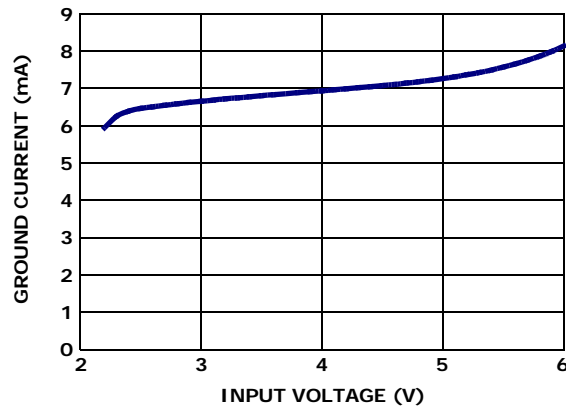
FIGURE 5. GROUND CURRENT vs SUPPLY VOLTAGE
