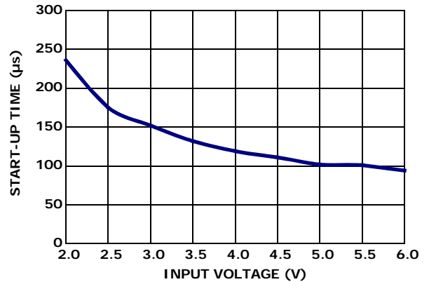
FIGURE 17. START-UP TIME vs SUPPLY VOLTAGE
