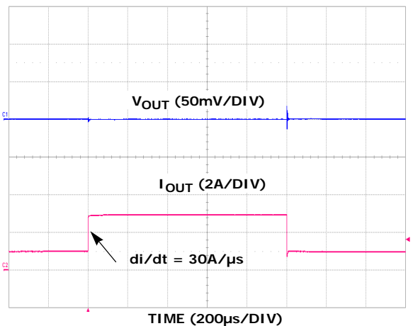
FIGURE 31. LOAD TRANSIENT 1A TO 3A, C_{OUT} = 10\mu F CERAMIC + 100µF OSCON
