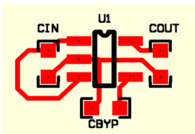
Figure 4. Fixed Mode
