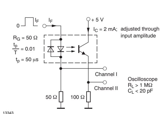
Figure 1. Test circuit, non-saturated operation
