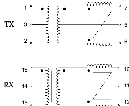
Schematic
