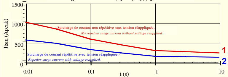
Fig.3: Surcharge de courant : I_{sm}(A_{peak}) = f(t) pour modèle 75A/ Surge current : I_{sm}(A_{peak}) = f(t) for 75A
