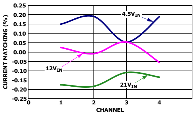
FIGURE 6. CHANNEL-TO-CHANNEL CURRENT MATCHING
