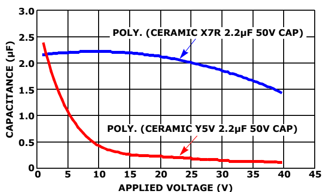
FIGURE 25. X7R AND Y5V TYPES CERAMIC CAPACITORS
