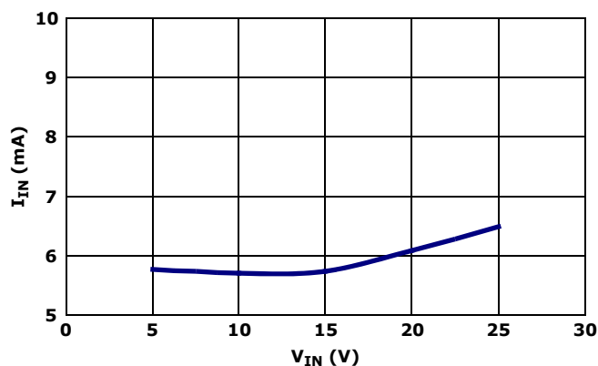
FIGURE 8. QUIESCENT CURRENT vs V_{IN} WITH PART ENABLED
