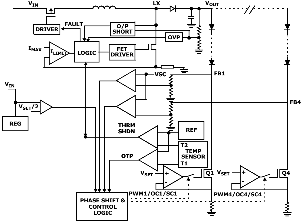
FIGURE 24. SIMPLIFIED FAULT PROTECTIONS
