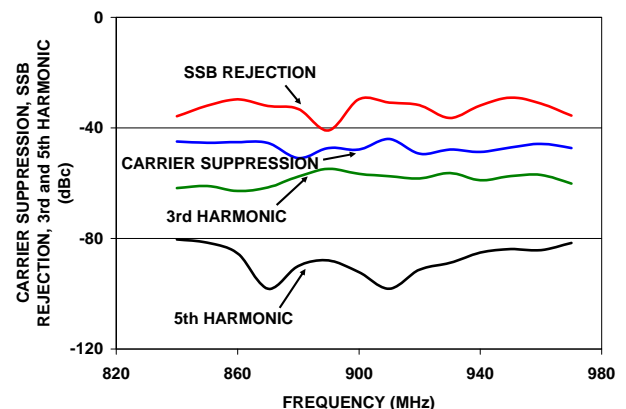
Carrier Suppression, SSB Rejection, 3rd and 5th Harmonic Suppression: V_{CC} = 2.85\text{V} , PLO = -2 dBm
