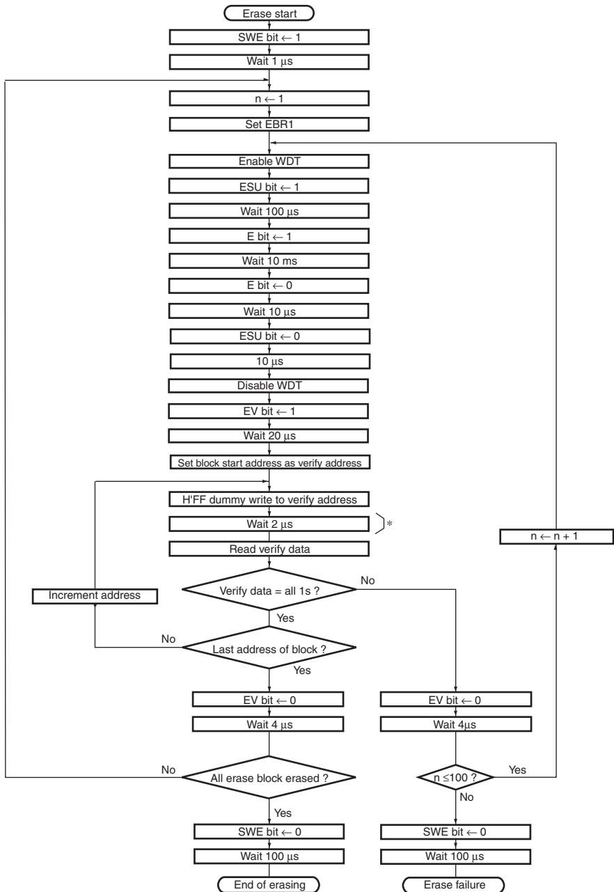
Figure 7.5 Erase/Erase-Verify Flowchart
