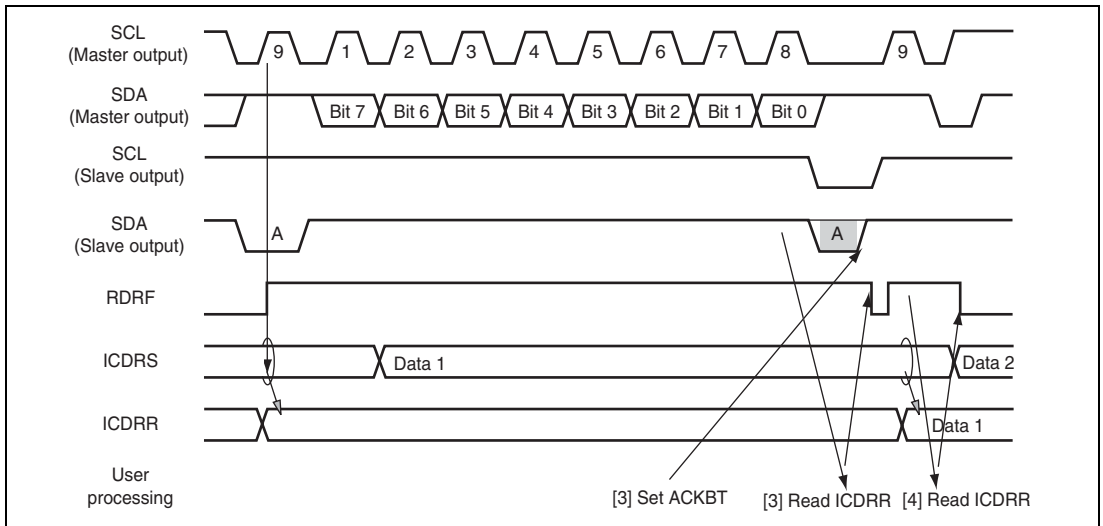
Figure 21.12 Slave Receive Mode Operation Timing (2)
