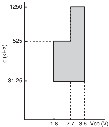
Figure 25.10 Power Supply Voltage and Operating Frequency Range (1)
