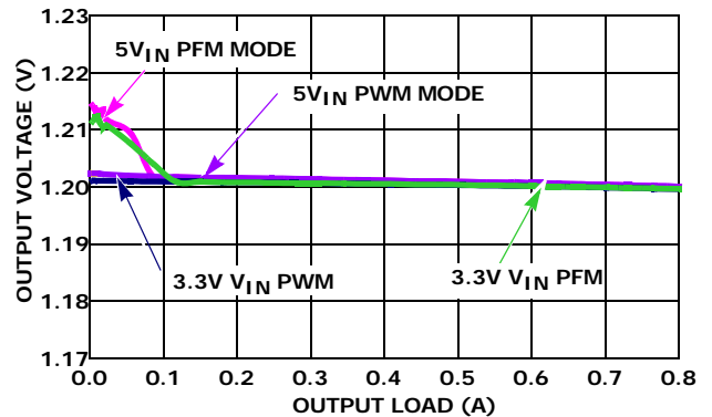
FIGURE 6. V_{OUT} REGULATION vs LOAD 2.25MHz 1.2VOUT PFM
