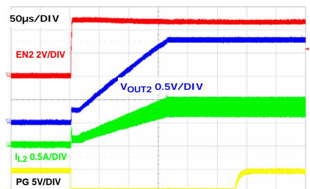
FIGURE 28. SOFT-START AT FULL LOAD CHANNEL 2
