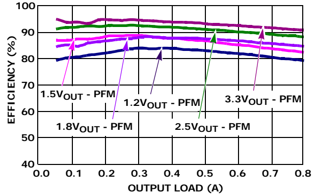
FIGURE 4. EFFICIENCY vs LOAD 2.25MHz 5VIN PFM
