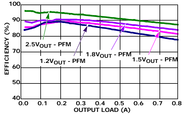
FIGURE 2. EFFICIENCY vs LOAD 2.25MHz 3.3VIN PFM
