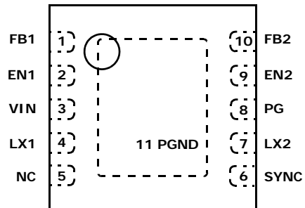
ISL8088 (10 LD 3X3 DFN) TOP VIEW
