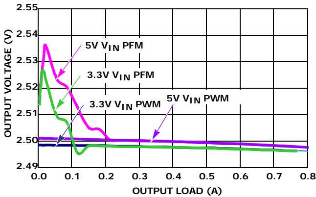
FIGURE 9. V_{OUT} REGULATION vs LOAD 2.25MHz 2.5V_{OUT}
