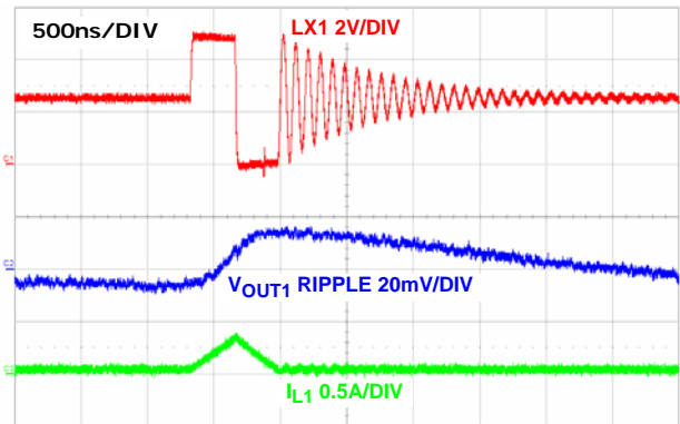
FIGURE 15. STEADY STATE OPERATION AT NO LOAD CHANNEL 1 (PFM)
