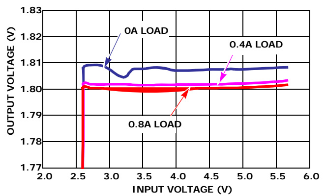
FIGURE 12. OUTPUT VOLTAGE REGULATION vs V_{IN} 1.8V_{OUT} PFM MODE
