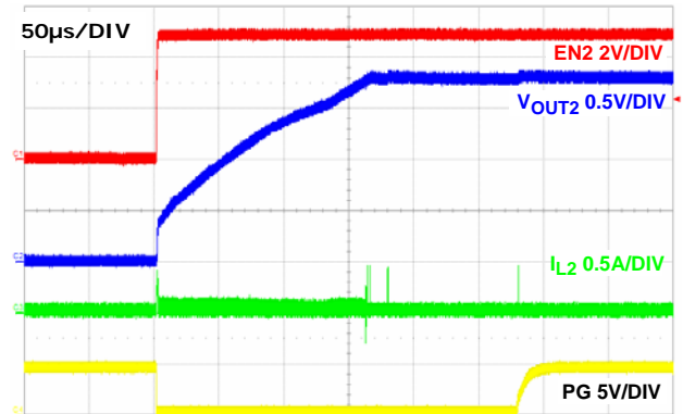
FIGURE 26. SOFT-START AT NO LOAD CHANNEL 2 (PFM)
