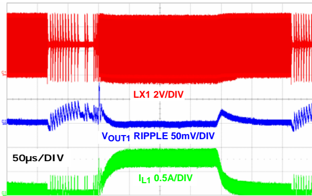
FIGURE 21. LOAD TRANSIENT CHANNEL 1 (PFM)
