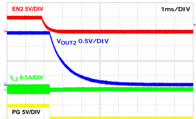
FIGURE 30. SOFT-DISCHARGE SHUTDOWN CHANNEL 2
