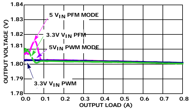
FIGURE 8. V_{OUT} REGULATION vs LOAD 2.25MHz 1.8V_{OUT}
