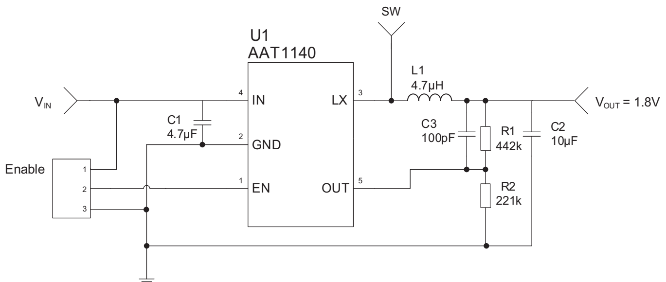
Figure 5: AAT1140 Adjustable Evaluation Board Schematic.
