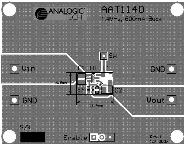
Figure 2: AAT1140 Evaluation Board Component Side Layout.
