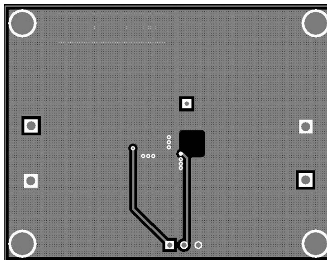
Figure 4: AAT1140 Evaluation Board Solder Side Layout.
