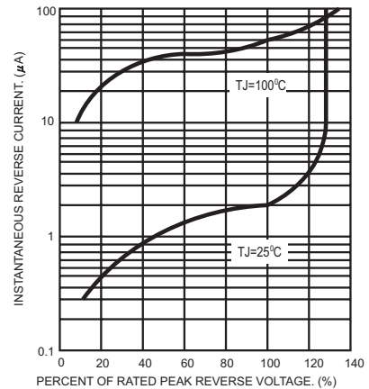
FIG.6- TYPICAL REVERSE CHARACTERISTICS
