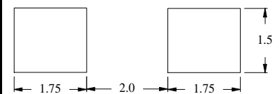
Recommended Soldering Pad Layout
