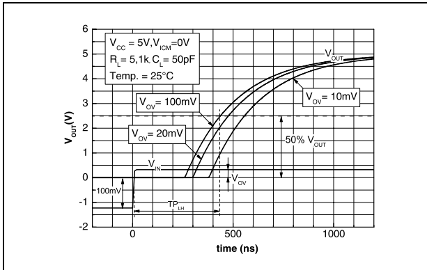
Figure 7. Response time versus overdrive with positive transition
