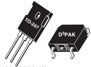
APT30GS60BRDQ2(G) APT30GS60SRDQ2(G)
