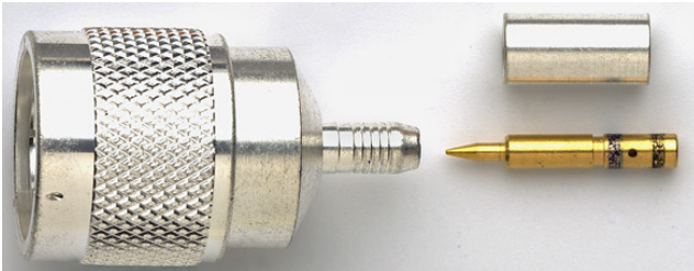
Model 7057 N (M) Crimp 50 \Omega
