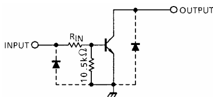
TD62593AFNG, TD62594AFNG
