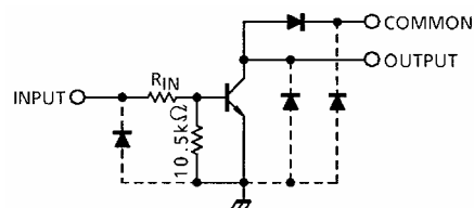
TD62597AFNG, TD62598AFNG
