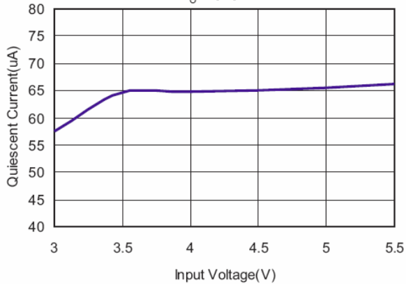
V_o = 3.3V
