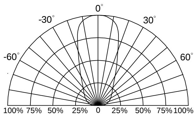
Fig.6 Directivity Radiation
