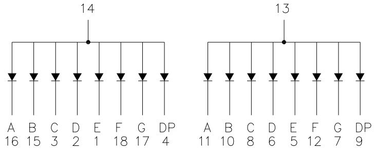
CSS-822 Common Anode. (CSS-823 is Common Cathode.)
