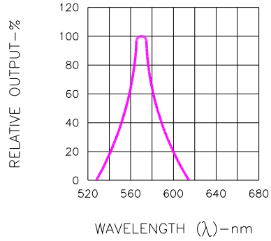
Fig.2 SPECTRAL RESPONSE
