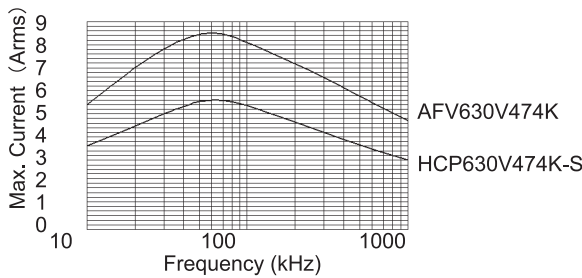
Current withstand comparison vs. HCP
