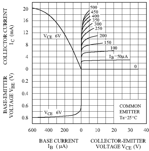
STATIC CHARACTERISTICS
