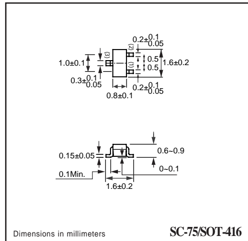
SC-75/SOT-416
