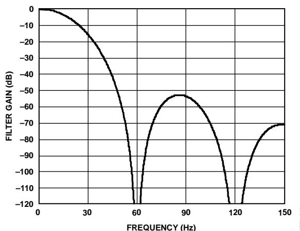
Figure 29. Sinc 4 Filter Response (FS[9:0] = 80)
