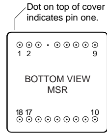
FIGURE 3: PIN OUT
