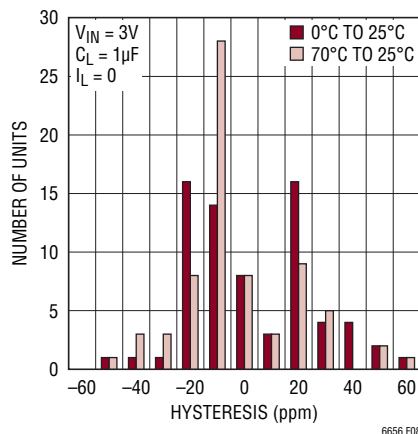
Figure 8. 0 ^\circ\text{C} to 70 ^\circ\text{C} Hysteresis
