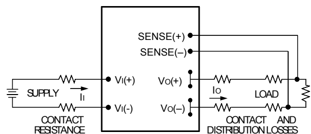
Figure 20. Effective Circuit Configuration for remote sense operation.
