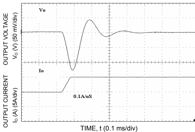
Figure 9. Transient Response to a Dynamic Load Change from 50% to 75% of full load at V_{in} = 24\text{ V} .
