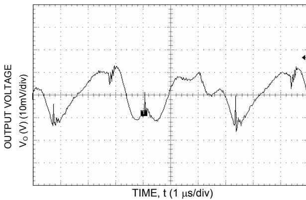
Figure 3. Typical Output Ripple and Noise at V_{IN} = 24\text{ V} .
