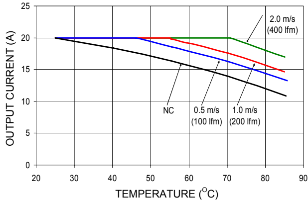
Figure 13. Thermal Derating Curves for the EQD020 module at 24Vin.
