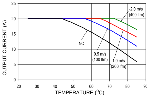
Figure 14. Thermal Derating Curves for the EQD020 module at 48Vin.
