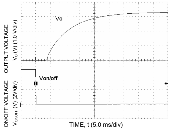
Figure 5. Typical Start-Up Characteristics from Remote ON/OFF at V_{in} = 18\text{ V} .
