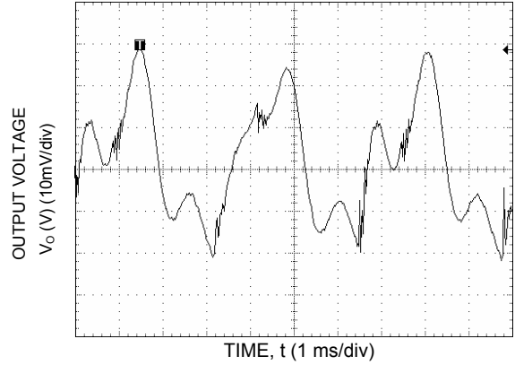
Figure 4. Typical Output Ripple and Noise at V_{IN} = 48\text{ V} .
