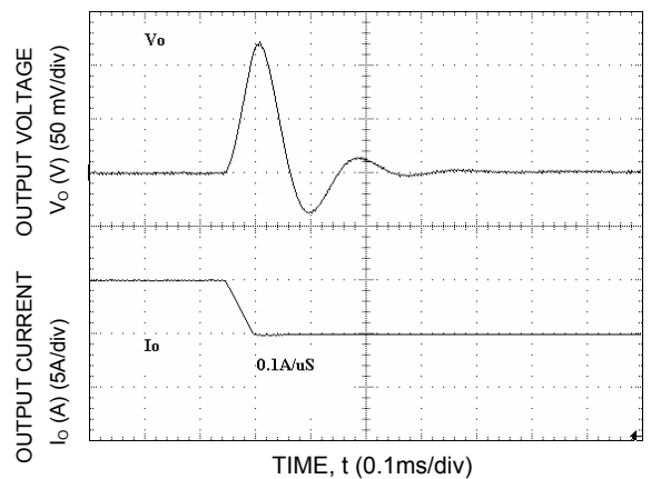
Figure 12. Transient Response to a Dynamic Load Change from 75% to 50% of full load at V_{in} = 48\text{ V} .
