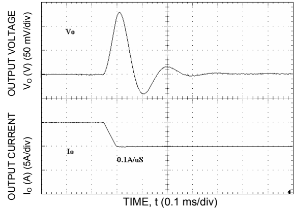
Figure 10. Transient Response to a Dynamic Load Change from 75% to 50% of full load at V_{in} = 24\text{ V} .
