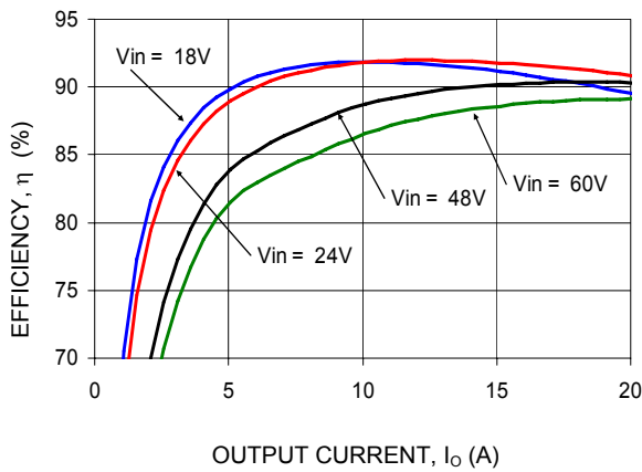
Figure 2. Typical Converter Efficiency versus Output Current.
