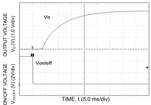
Figure 6. Typical Start-Up Characteristics from Remote ON/OFF at V_{in} = 48\text{ V} .
