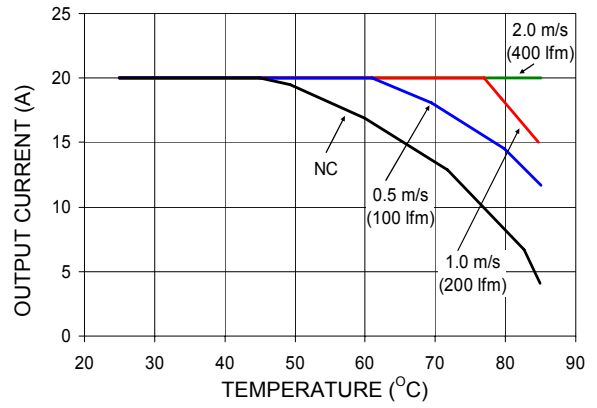
Figure 15. Thermal Derating Curves for the EQD020-H module with heat plate at 48Vin.
