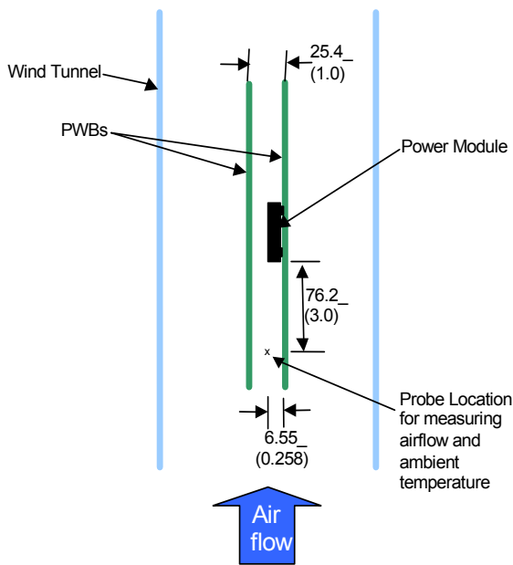
Figure 22. Thermal Test Set up.
