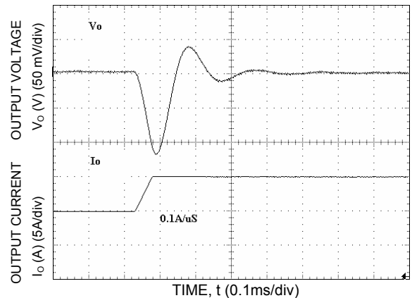
Figure 11. Transient Response to a Dynamic Load Change from 50% to 75% of full load at V_{in} = 48\text{ V} .
