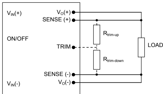
Figure 21. Circuit Configuration to program output voltage using an external resistor.
