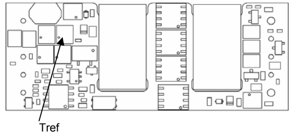
Figure 23. T_{ref} Temperature Measurement Location.
