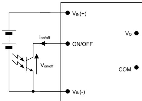
Figure 19. Circuit configuration for using Remote On/Off Implementation.
