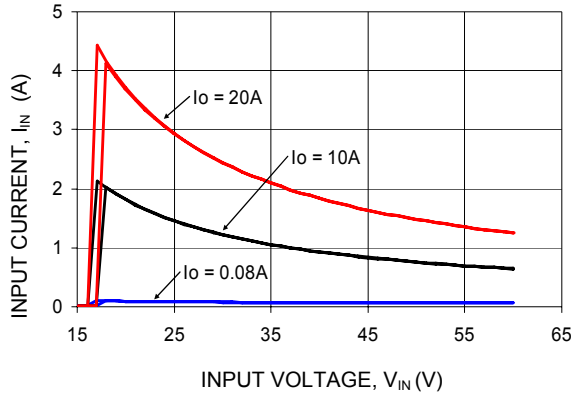
Figure 1. Typical Input characteristics.
