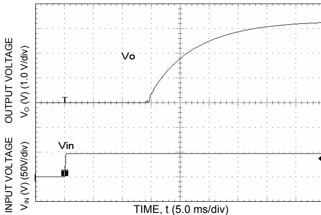
Figure 8. Typical Start-Up Characteristics using Input Voltage at V_{in} = 48\text{ V} .
