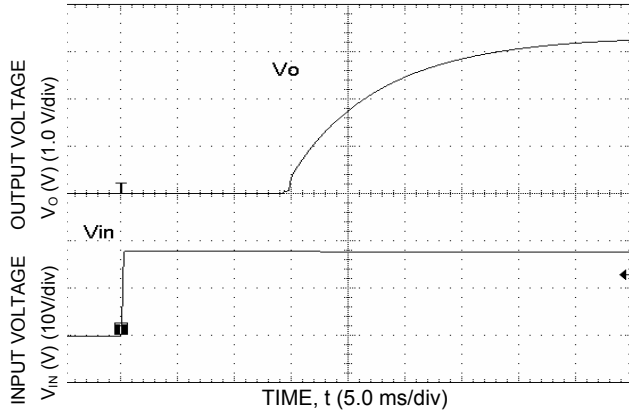
Figure 7. Typical Start-Up Characteristics using Input Voltage at V_{in} = 18\text{ V} .
