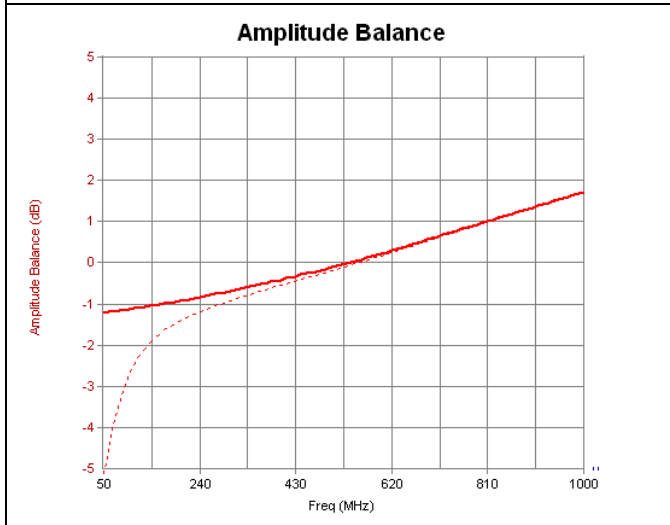
Figure 2 The Balun with an external inductor in a Ruthroff implementation with an external 100 nH inductor. Data is compared to the basic Guanella configuration (dashed lines). Other inductor values can be used with different results.
