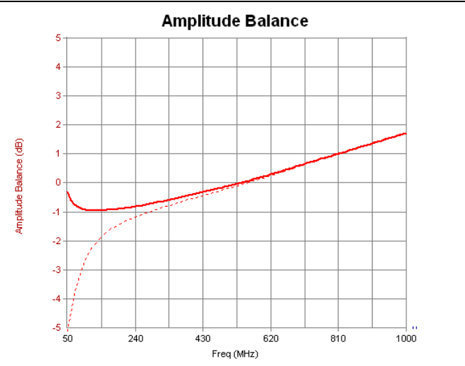
Figure 3 The Balun with an external inductor in a Ruthroff implementation with an external 100 nH inductor and DC block to enhance insertion and return loss. Data is compared to the basic Guanella configuration (dashed lines). Other capacitor and inductor values can be used with different results.
