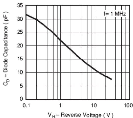
Figure 6. Diode Capacitance vs. Reverse Voltage
