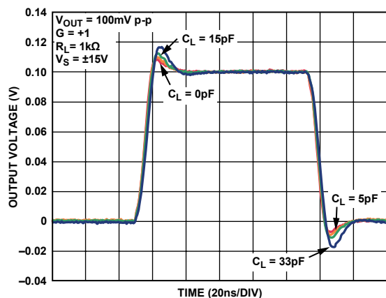
Figure 22. Small Signal Transient Response for Various Capacitive Loads
