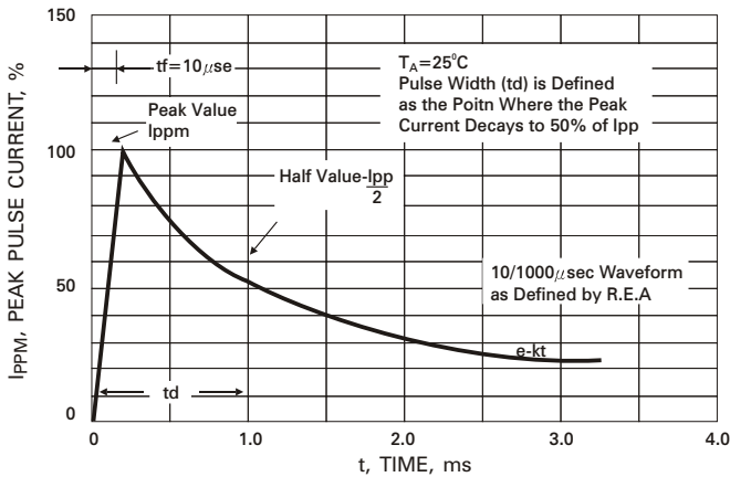
Fig. 3 - PULSE WAVEFORM
