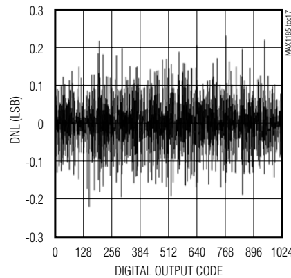
DIFFERENTIAL NONLINEARITY
