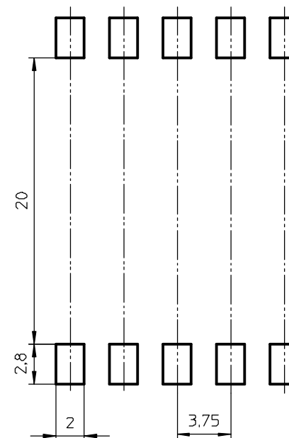
PROPOSED PAD ARRANGEMENT:
