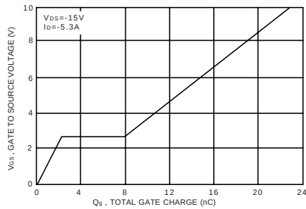
Figure 3. Gate Charge
