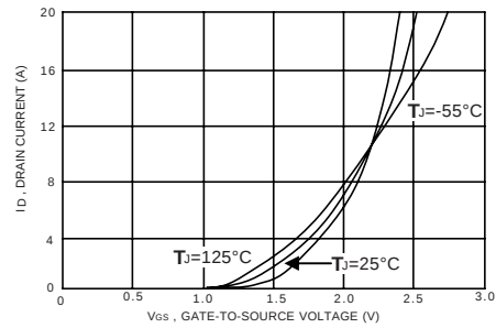
Figure 2. Transfer Characteristics
