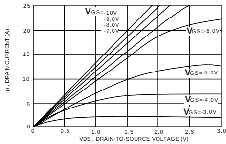
Figure 1. Output Characteristics
