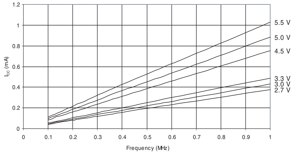
Figure 30-3. Active Supply Current vs. frequency (1 - 20 MHz) - Temp.=25°C
