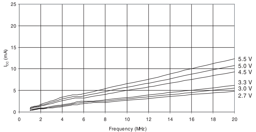
Figure 30-4. Active Supply Current vs. frequency (1 - 20 MHz) - Temp.=125°C
