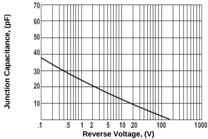
Fig.5-Typical Junction Capacitance
