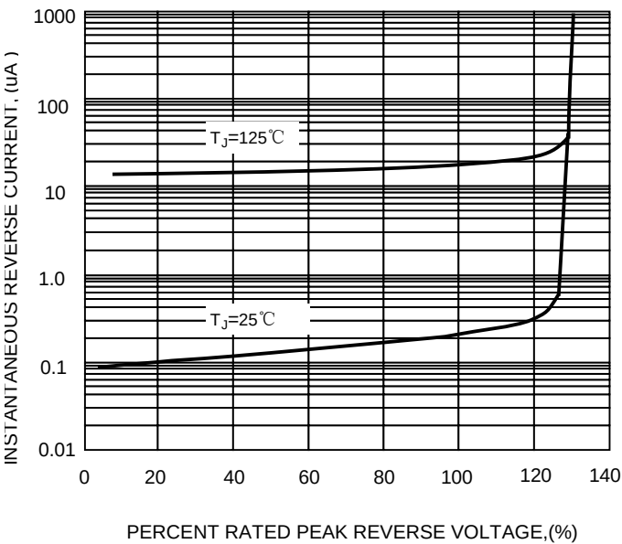
FIG.4-TYPICAL REVERSE CHARACTERISTICS
