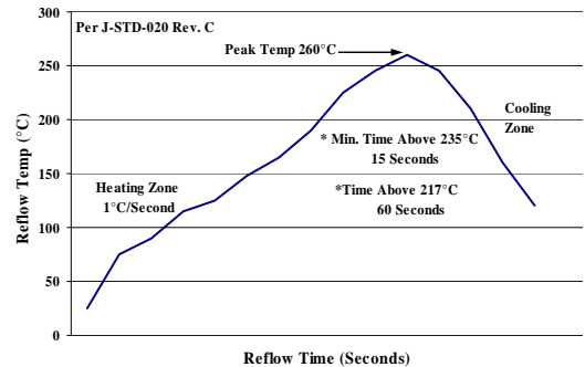
Figure 25. Recommended linear reflow profile using Sn/Ag/Cu solder.
