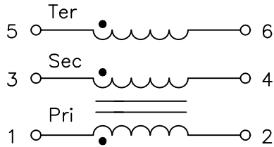
3 Windings
