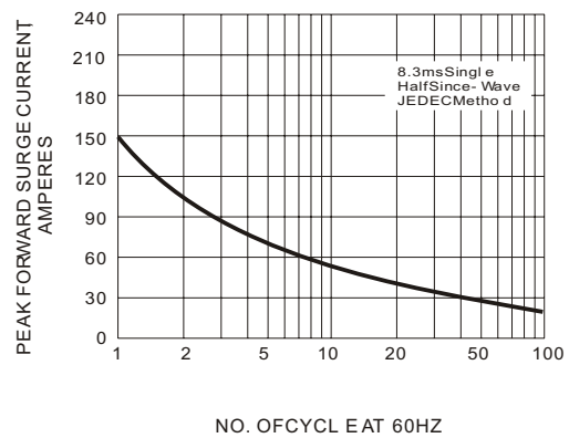
Fig.4- TMAXIMUM NON - REPETITIVE SURGE CURRENT
