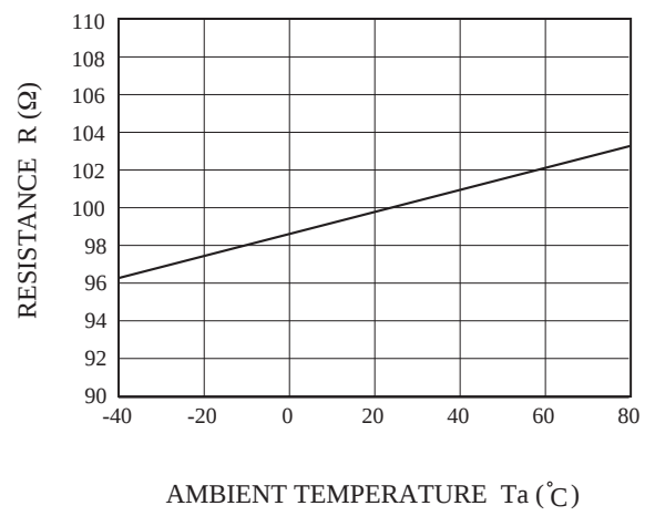
R_{Line} - TEMPERATURE
