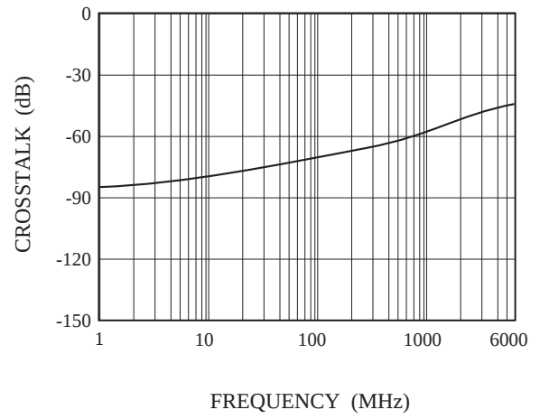
ANALOG CROSSTALK
