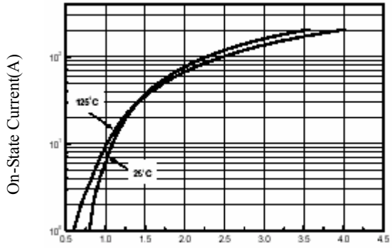
FIGURE 3-Typical Forward Voltage(V)
