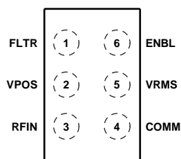
ADL5504 TOP VIEW (BALL SIDE DOWN) Not to Scale
