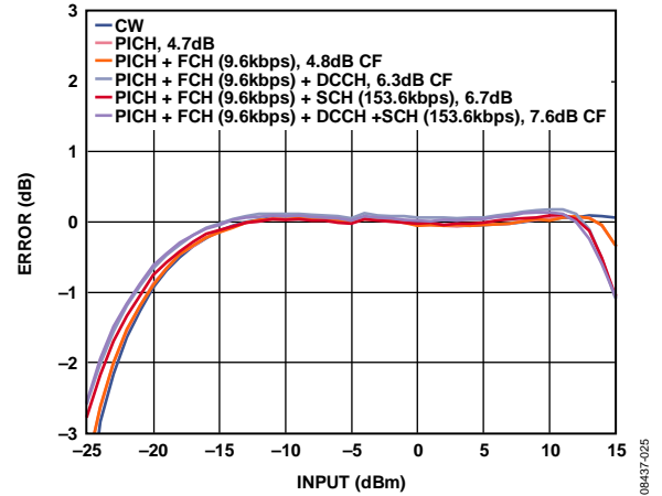
Figure 25. Error from CW Linear Reference vs. Input with Various CDMA2000 Reverse Link Waveforms at 1900 MHz, C_{FLTR} = 12 nF, C_{OUT} = Open
