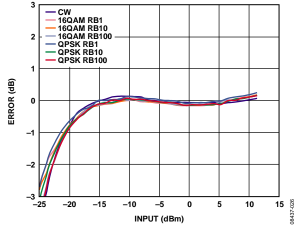
Figure 26. Error from CW Linear Reference vs. Input with Various LTE Reverse Link Waveforms at 2600 MHz, C_{FLTR} = 12 nF, C_{OUT} = Open
