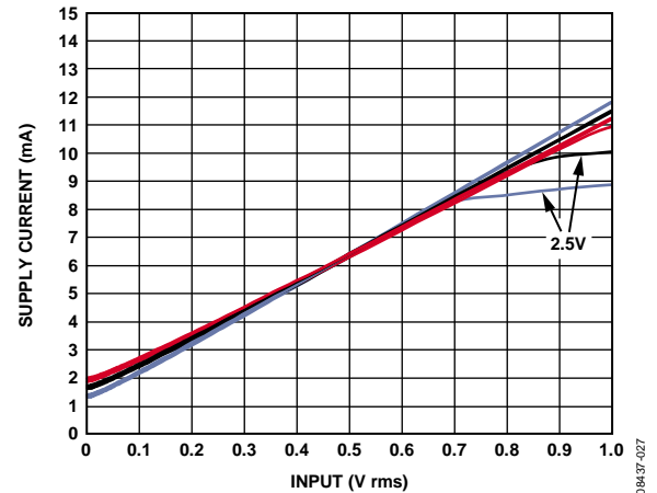
Figure 27. Supply Current vs. Input Level, 2.5 V, 3.0 V, and 3.3 V Supplies, 900 MHz Frequency, at -40°C, +25°C, and +85°C
